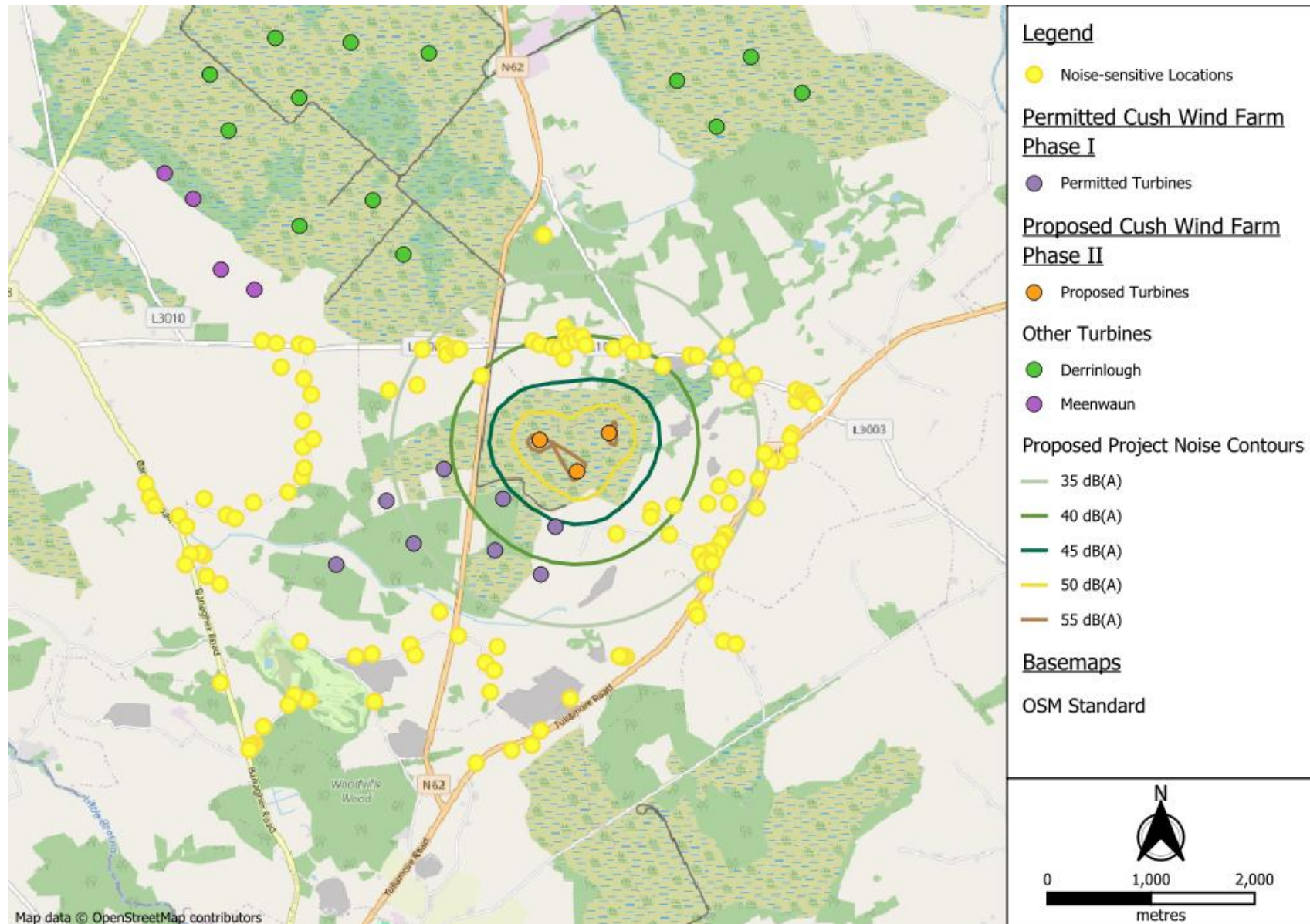
Figure 12-7-1. Noise Contours for Proposed Development
