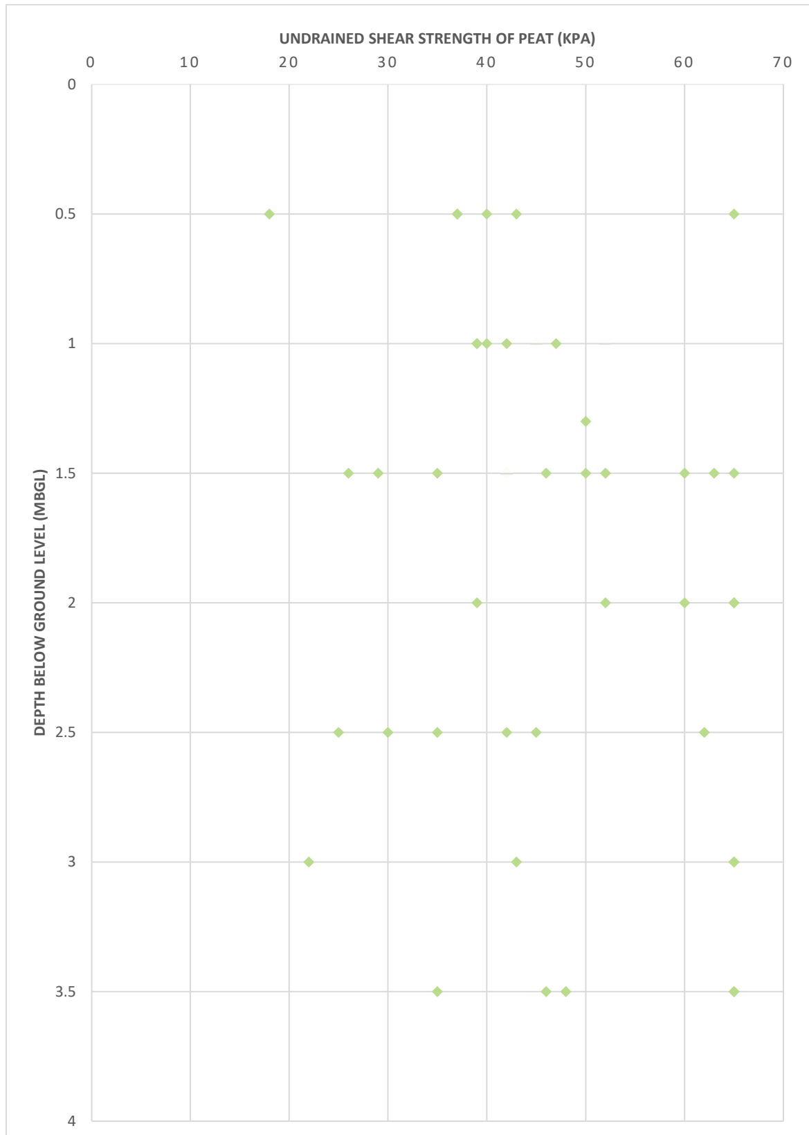
Figure 5-1: Undrained Shear Strength ( c_u ) Profile for Peat with Depth
